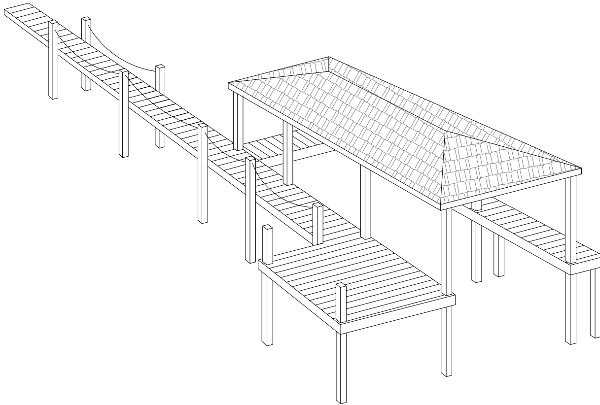
Basic Dock & Boat House
